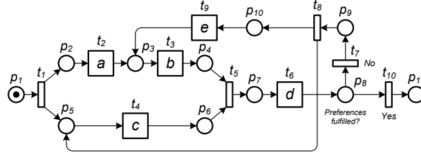
Fig. 2. A net system that captures the semantics of the BPMN model in Fig. 1
